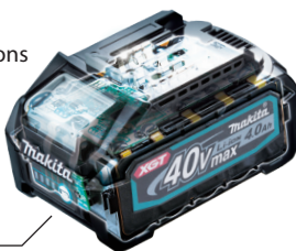
Terminal short-circuit prevention structure
